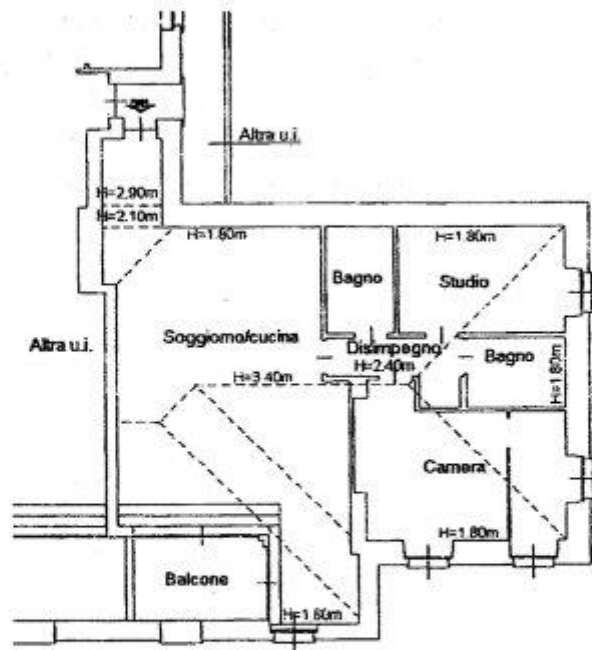
PIANO QUARTO
