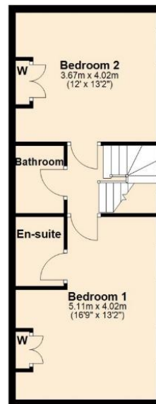
First Floor Approx. 45.5 sq. metres (489.4 sq. feet)
