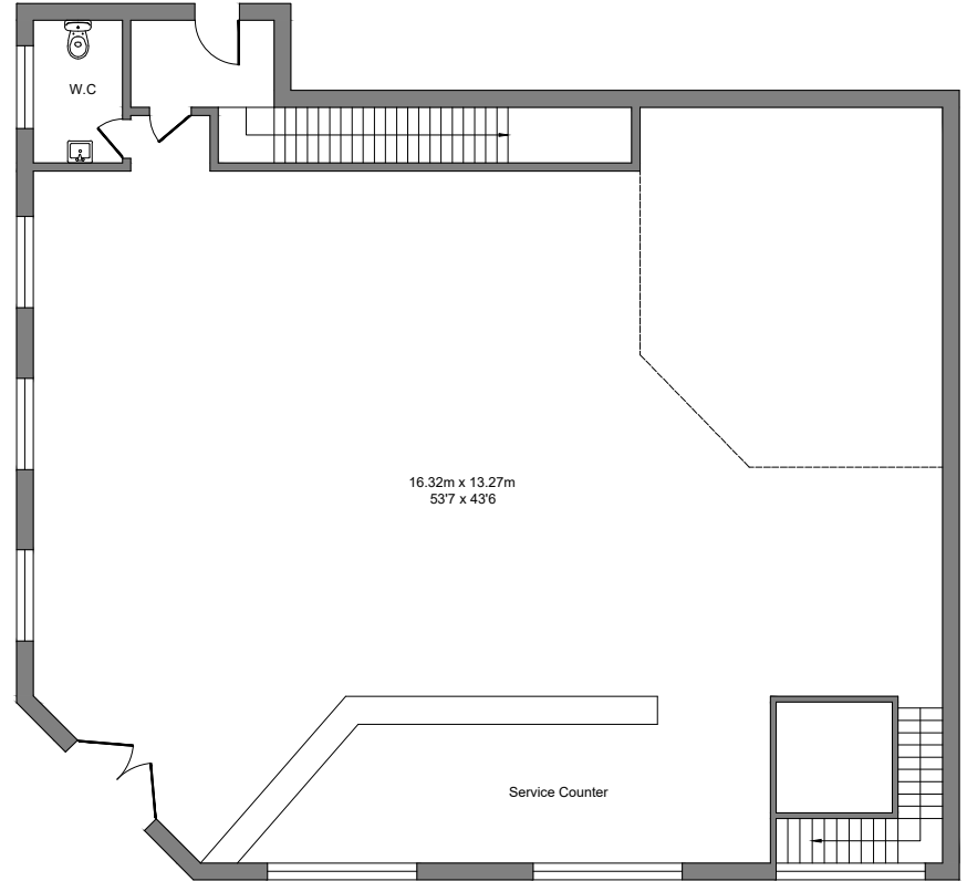
2 Ground Floor Plan
