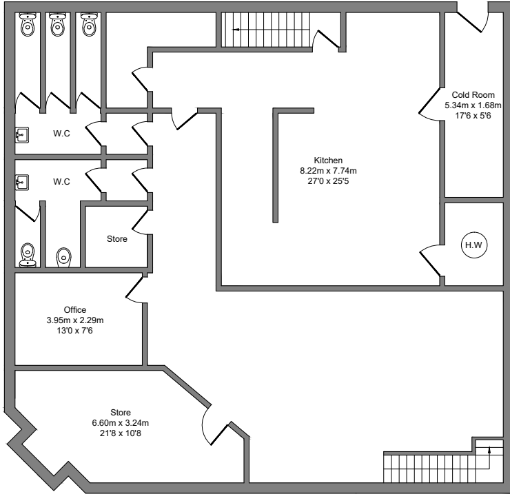
1 Lower Ground Floor Plan
