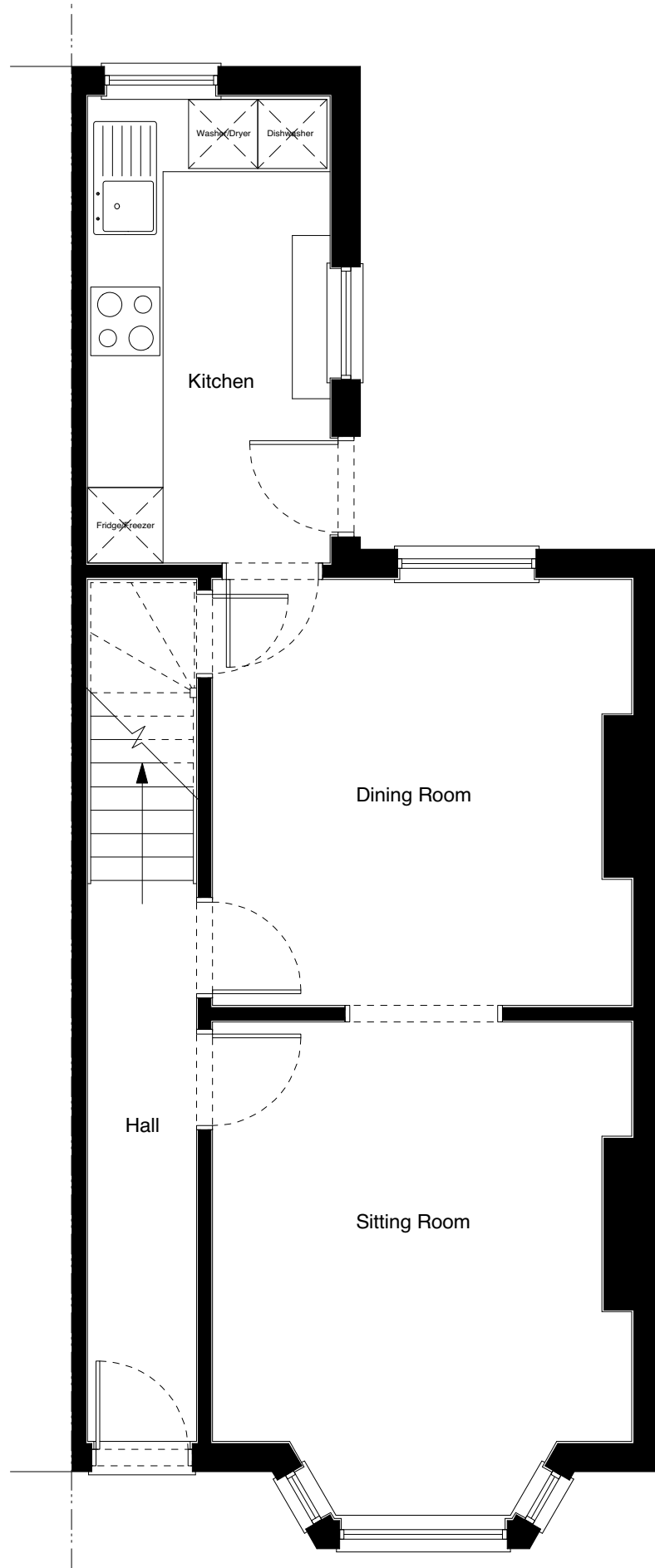
16 Hillside Street (Scale 1:50@A3)
